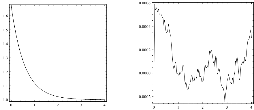
Figure 12: Course of the functional M_{11}(t) , Hard Spheres
