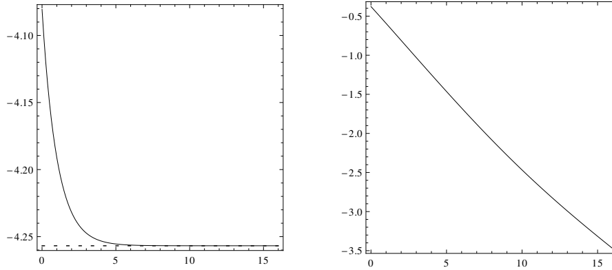
Figure 8: Course of the H -functional and of the L_2 -error for n = 343
