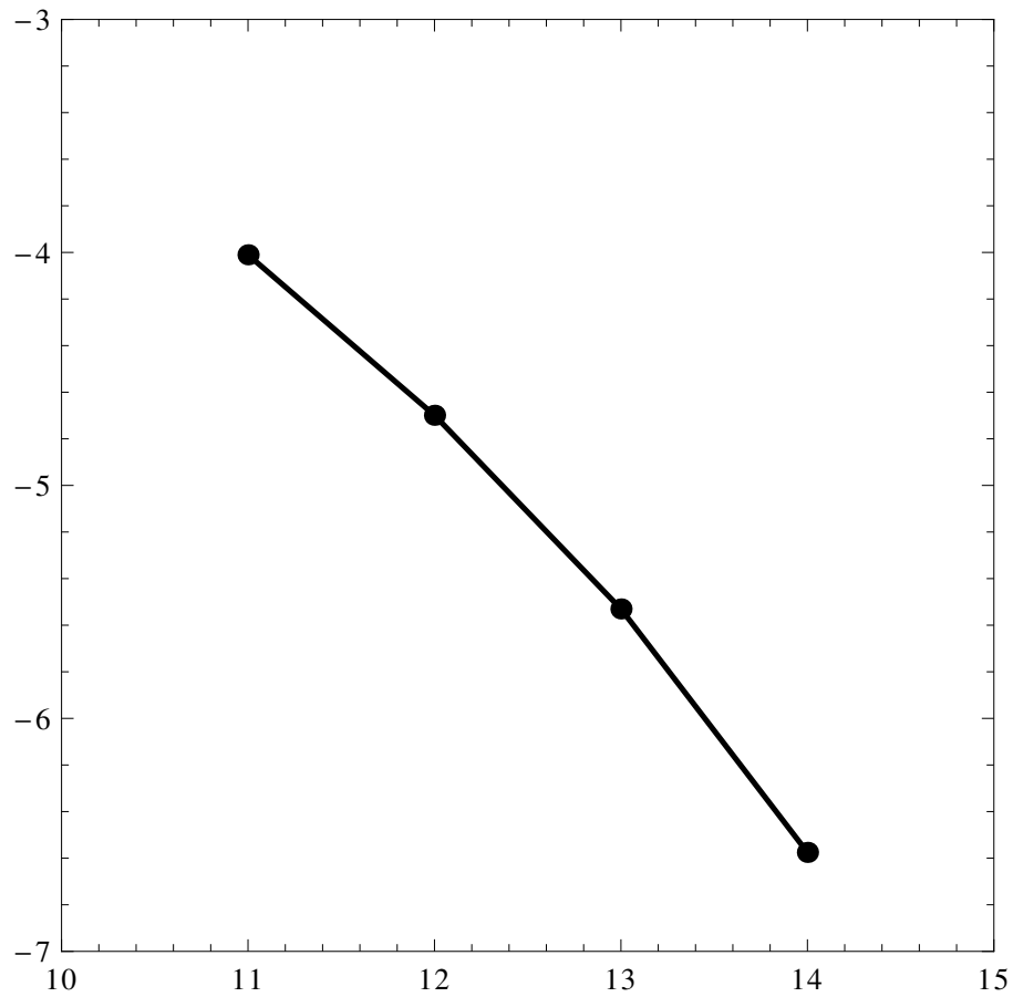
Figure 10: \log_{10} course of the L_2(\mathbb{R}^3) error, BKW
