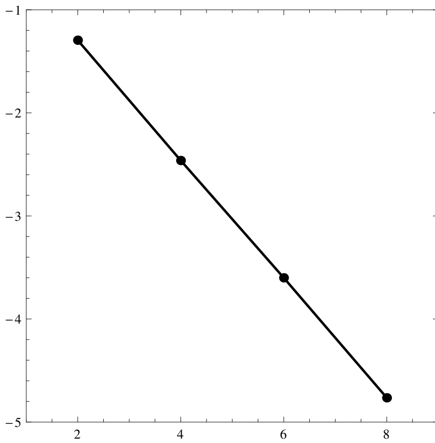
Figure 3: \log_{10} course of the L_2(\mathbb{R}^3) error
