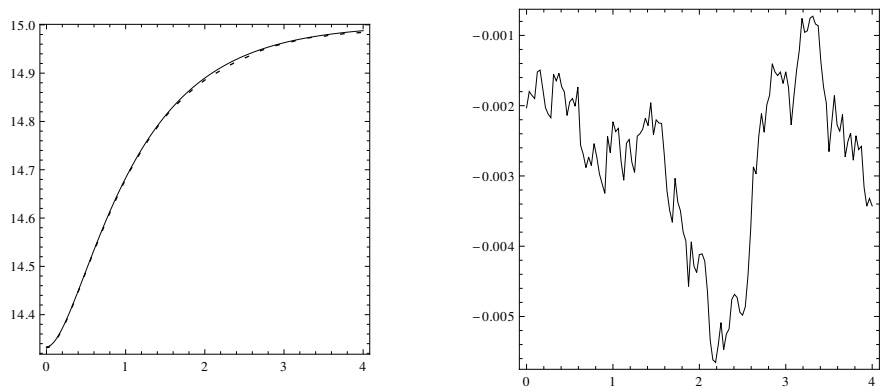
Figure 13: Course of the functional s(t) , Hard Spheres
