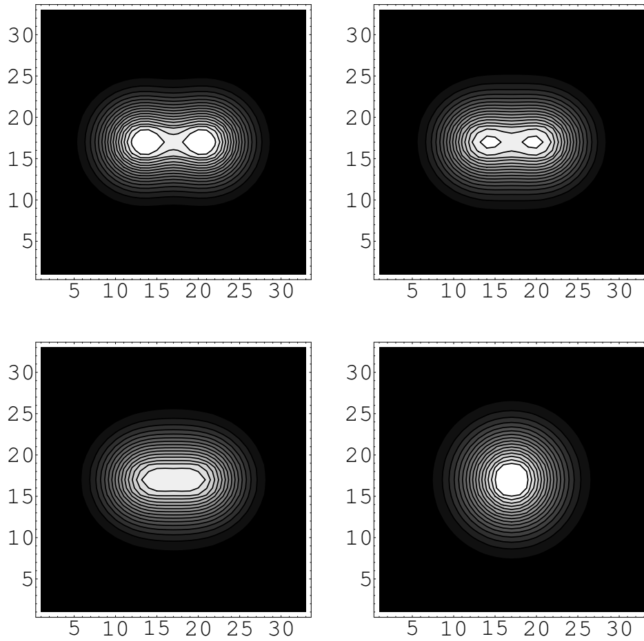
Figure 7: Contours of the density function for t = 0, 1/4, 1, 16
