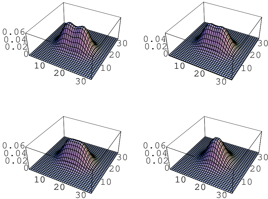
Figure 6: Density function for t = 0, 1/4, 1, 16
