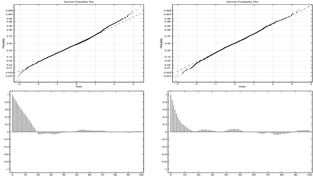
Figure 4.5 Goodness of fit of the 20-days-ahead conditional distribution of GED EGARCH(1,1) model. The data analyzed are \tilde{z}_t^{(20)} , the 20-day returns transformed with the conditional cdf specified by (2.1) and (2.3) and the inverse of the standard normal cdf. Top: The normal plot of the data obtained in Setup 1 (Left) and Setup 2 (Right). Bottom: The sample ACF of data (Setup 2)(Left) and absolute values (Right).
