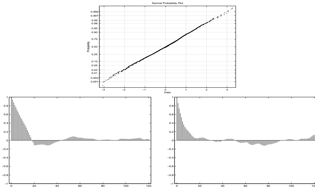
Figure 4.6 Goodness of fit of the 20-days-ahead conditional distribution of the regression model. The data analyzed are \tilde{z}_t^{(20)} , the 20-day returns transformed with the conditional cdf specified by (2.4) and the inverse of the standard normal cdf. Top: The normal plot of the data. Bottom: The sample ACF of data (Setup 2)(Left) and absolute values (Right).
