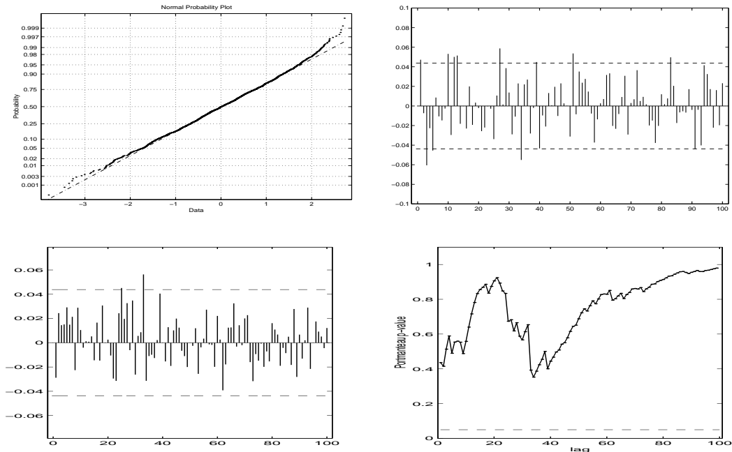
Figure 4.1 Goodness of fit of the 1-day-ahead conditional distribution of Student's t GARCH(1,1) model. The data analyzed are \tilde{z}_t^{(1)} (4.4), i.e. daily returns transformed with the conditional cdf specified by (2.1) and (2.2) and the inverse of the standard normal cdf. Top: The normal probability plot (Left). The sample ACF of the data (Right). Bottom: The sample ACF of the absolute values (Left). The Portmanteau test for the absolute values (Right).
