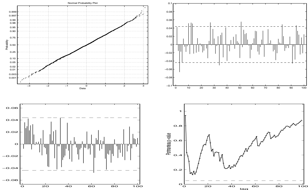
Figure 4.3 Goodness of fit of the 1-day-ahead conditional distribution of the regression model. The data analyzed are \tilde{z}_t^{(1)} (4.4), i.e. daily returns transformed with the conditional cdf specified by (2.4) and the inverse of the standard normal cdf. Top: The normal probability plot (Left). The sample ACF of the data (Right). Bottom: The sample ACF of the absolute values (Left). The Portmanteau test for the absolute values (Right).
