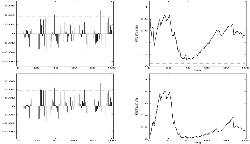
Figure 3.5 Sample ACF (Left) and Portmanteau test (Right) for the absolute values of the estimated innovations ( \hat{\epsilon}_t ) of the Student's t GARCH(1,1) (Top) and of the GED EGARCH(1,1) (Bottom) fit to the series of S&P 500 returns.
