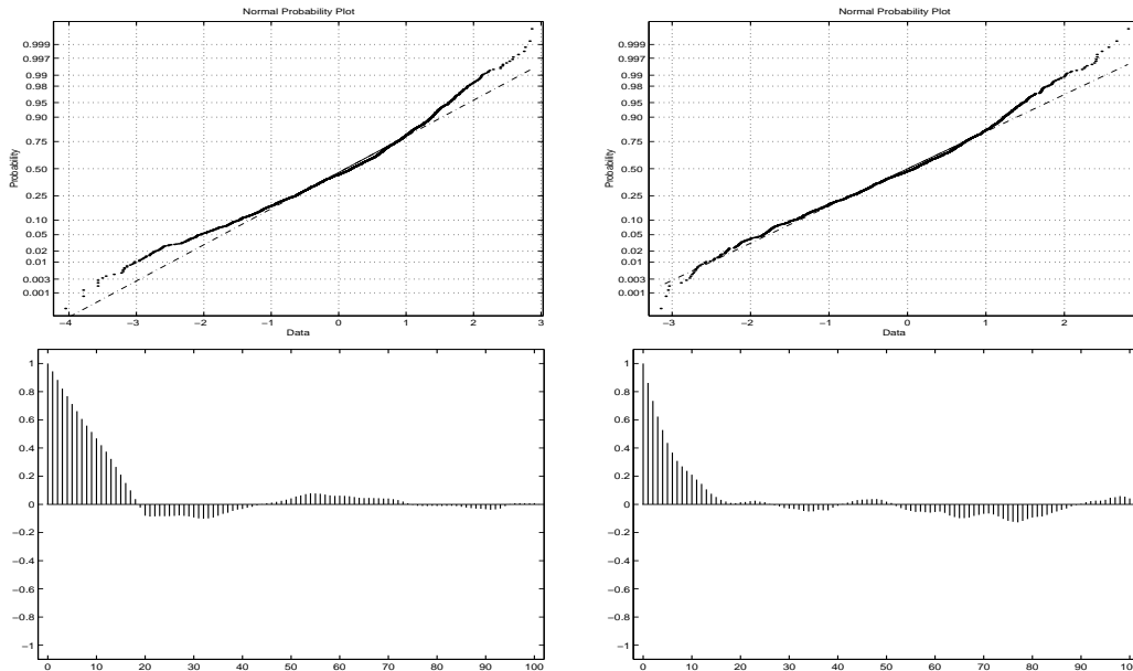
Figure 4.4 Goodness of fit of the 20-days-ahead conditional distribution of Student's t GARCH(1,1) model. The data analyzed are \tilde{z}_t^{(20)} , the 20-day returns transformed with the conditional cdf specified by (2.1) and (2.2) and the inverse of the standard normal cdf. Top: The normal plot of the data obtained in Setup 1 (Left) and Setup 2 (Right). Bottom: The sample ACF of data (Setup 2)(Left) and absolute values (Right).
