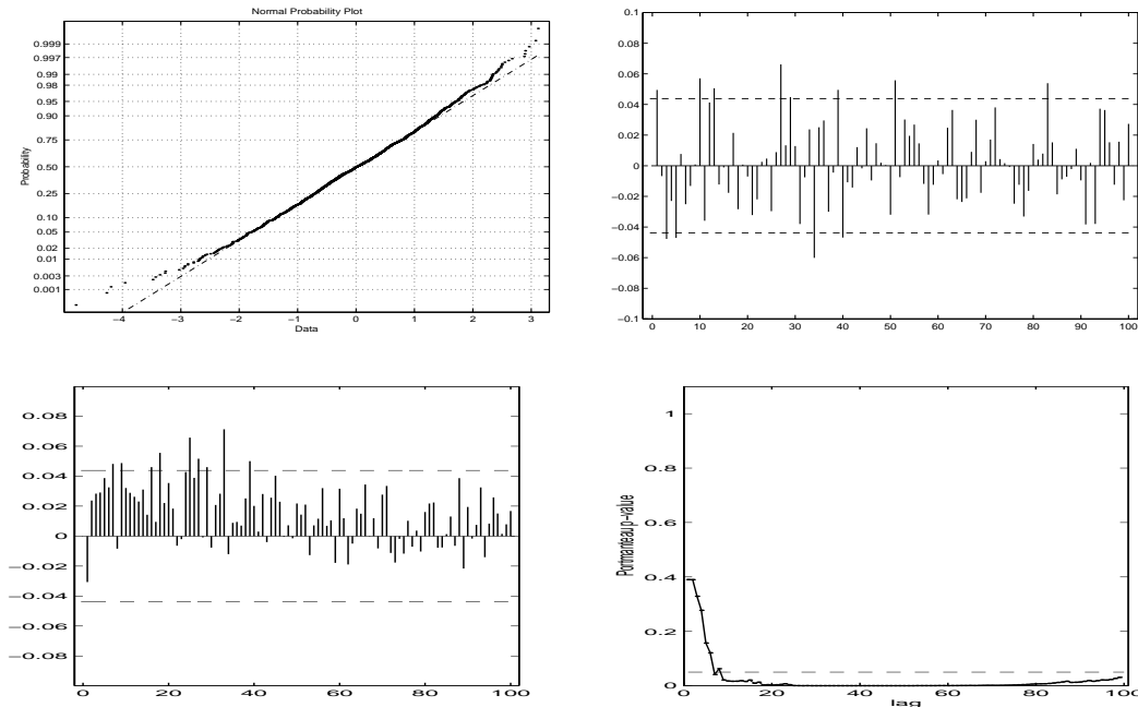
Figure 4.2 Goodness of fit of the 1-day-ahead conditional distribution of GED-EGARCH(1,1) model. The data analyzed are \tilde{z}_t^{(1)} (4.4), i.e. daily returns transformed with the conditional cdf specified by (2.1) and (2.3) and the inverse of the standard normal cdf. Top: The normal probability plot (Left). The sample ACF of the data (Right). Bottom: The sample ACF of the absolute values (Left). The Portmanteau test for the absolute values (Right).
