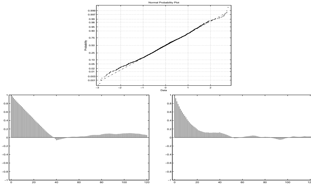
Figure 4.9 Goodness of fit of the 40-days-ahead conditional distribution of the regression model. The data analyzed are \tilde{z}_t^{(40)} , the 40-day returns transformed with the conditional cdf specified by (2.4) and the inverse of the standard normal cdf. Top: The normal plot of the data. Bottom: The sample ACF of data (Left) and absolute values (Right).
