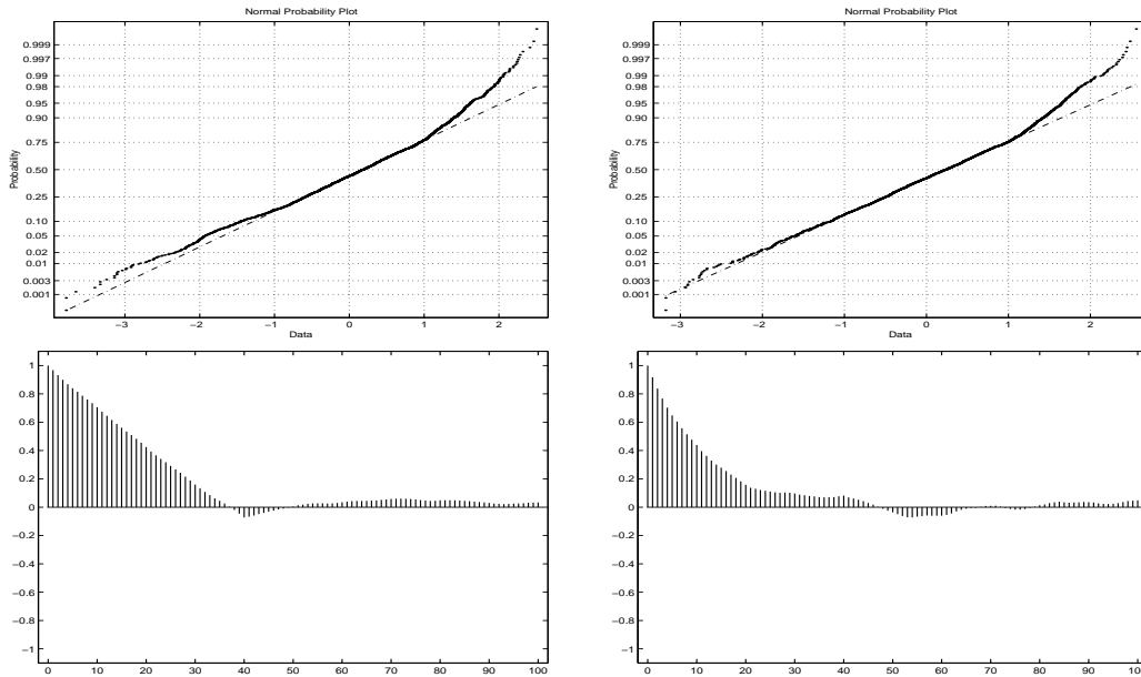
Figure 4.7 Goodness of fit of the 40-days-ahead conditional distribution of Student's t GARCH(1,1) model. The data analyzed are \tilde{z}_t^{(40)} , the 40-day returns transformed with the conditional cdf specified by (2.1) and (2.2) and the inverse of the standard normal cdf. Top: The normal plot of the data obtained in Setup 1 (Left) and Setup 2 (Right). Bottom: The sample ACF of data (Setup 2)(Left) and absolute values (Left).
