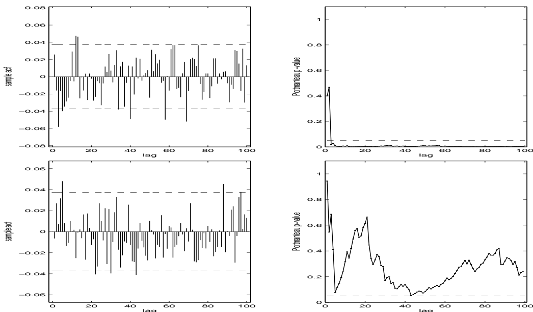
Figure 3.4 Sample ACF (Left) and Portmanteau test (Right) for the estimated innovations ( \hat{\varepsilon}_t ) of the regression model (2.4) fit to the series of S&P 500 returns (Top) and of their absolute values (Bottom).
