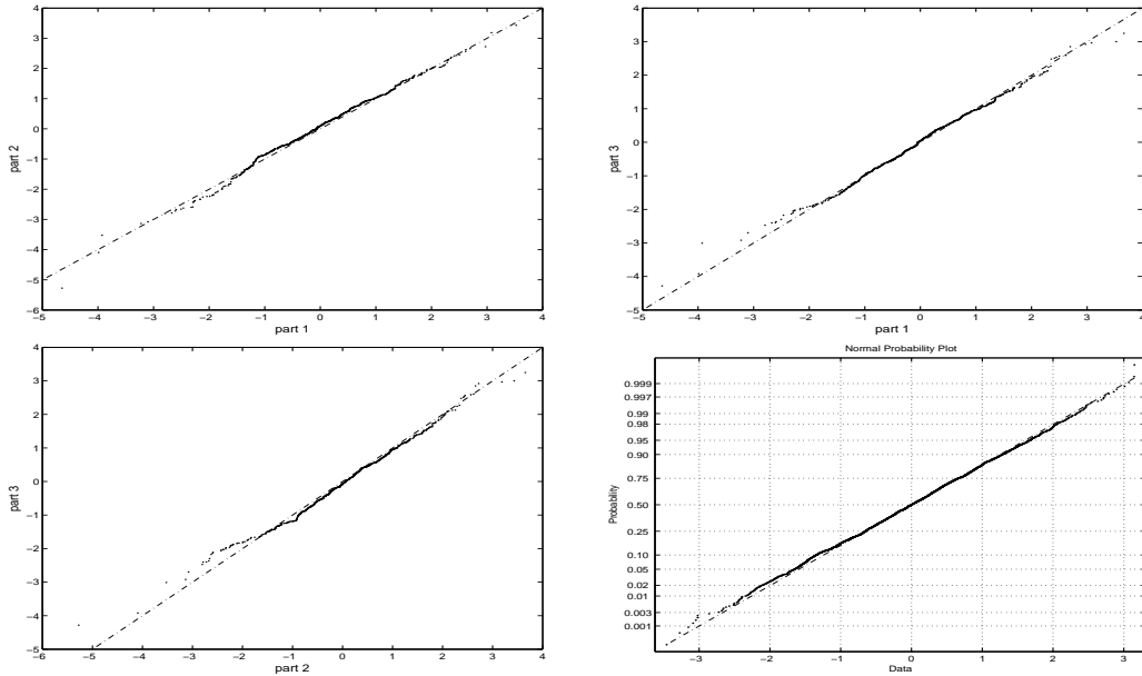
Figure 3.3 QQ-plots of the pairs of 3 periods of innovations (Top and Bottom Left). Normal probability plot of the innovations transformed with estimated asymmetric Pearson type VII cdf, \hat{F}^{VII} with the data on the x-axis and the normal quantile function on the y-axis (Bottom Right).
