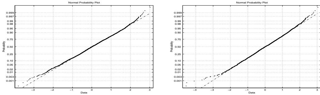
Figure 3.6 Normal probability plot of the innovations of the Student's t GARCH(1,1) transformed with estimated t cdf and the inverse of the standard normal cdf (Left) and of the innovations of the GED EGARCH(1,1) transformed with estimated GED cdf and the inverse of the standard normal cdf (Right) with the data on the x -axis and the normal quantile function on the y -axis (See (3.9)).
