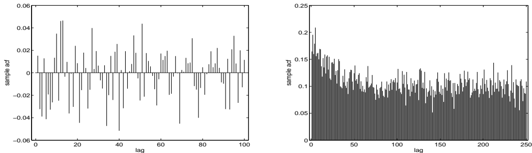
Figure 1.1 Sample ACF for S&P 500 returns (Left) and absolute returns (Right). Since the dependency structure in the data is unknown, no confidence intervals for the correlations are displayed.
