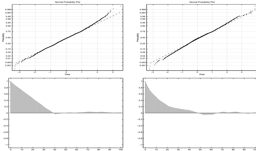
Figure 4.8 Goodness of fit of the 40-days-ahead conditional distribution of GED EGARCH(1,1) model. The data analyzed are \tilde{z}_t^{(40)} , the 40-day returns transformed with the conditional cdf specified by (2.1) and (2.3) and the inverse of the standard normal cdf. Top: The normal plot of the data obtained in Setup 1 (Left) and Setup 2 (Right). Bottom: The sample ACF of data (Setup 2)(Left) and absolute values (Right).
